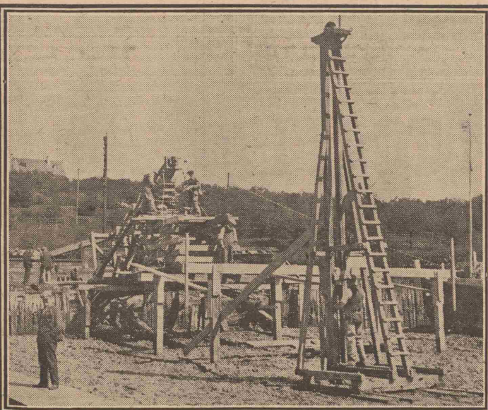
NEW THAMES BRIDGE.—Work on the building of a bridge at Canvey Island, Essex. It is to give access to Benfleet.
